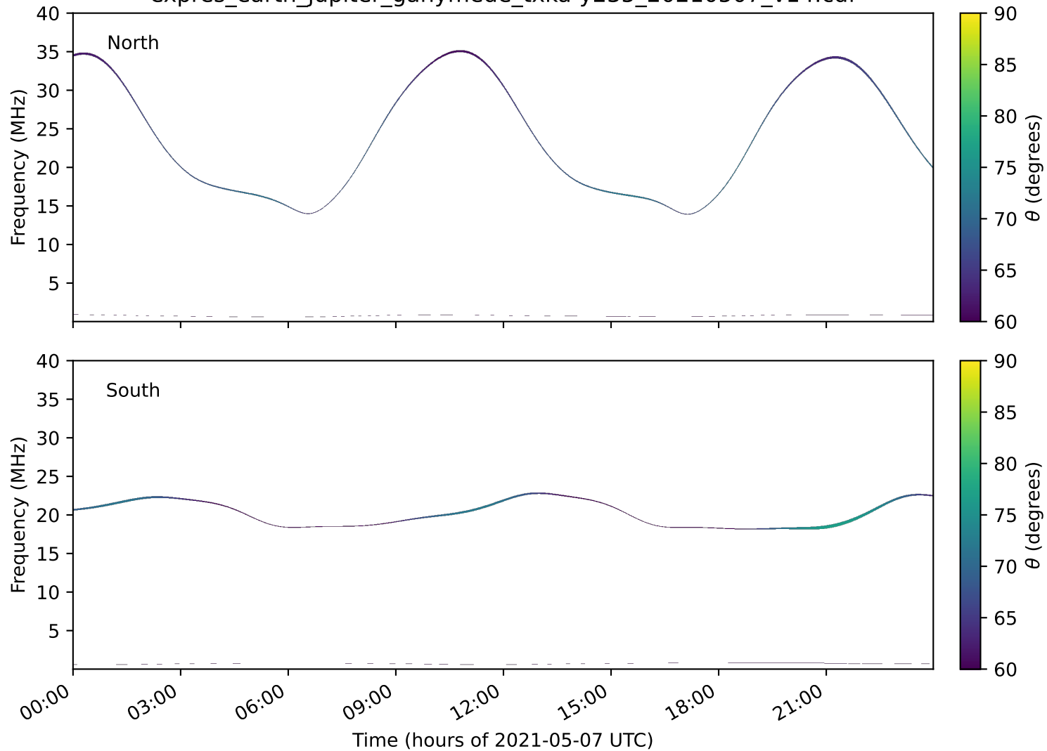
expres_earth_jupiter_ganymede_txka-y235_20210507_v14.cdf
