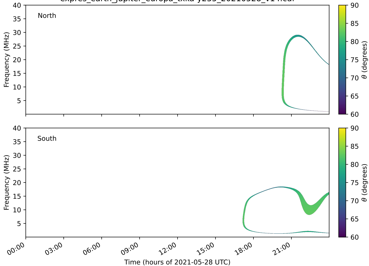
expres_earth_jupiter_europa_txka-y235_20210528_v14.cdf
