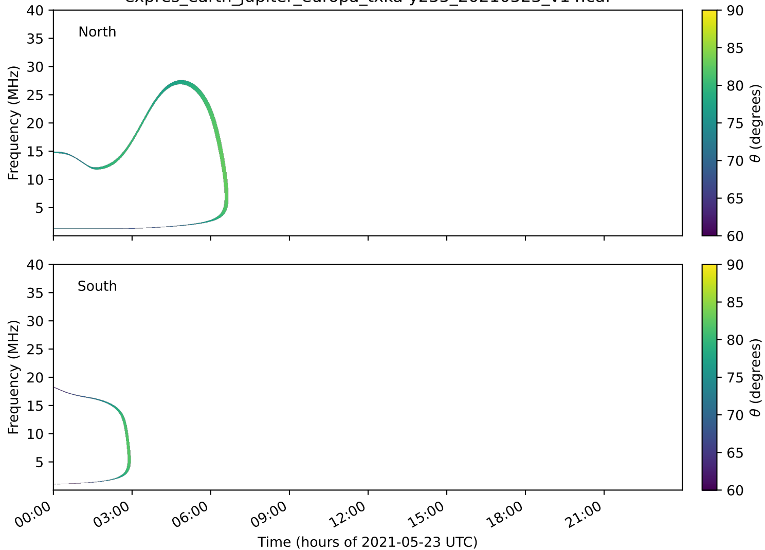
expres_earth_jupiter_europa_txka-y235_20210523_v14.cdf
