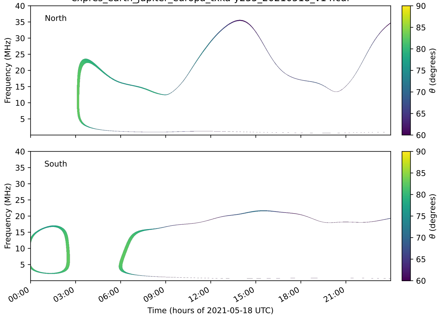
expres_earth_jupiter_europa_txka-y235_20210518_v14.cdf
