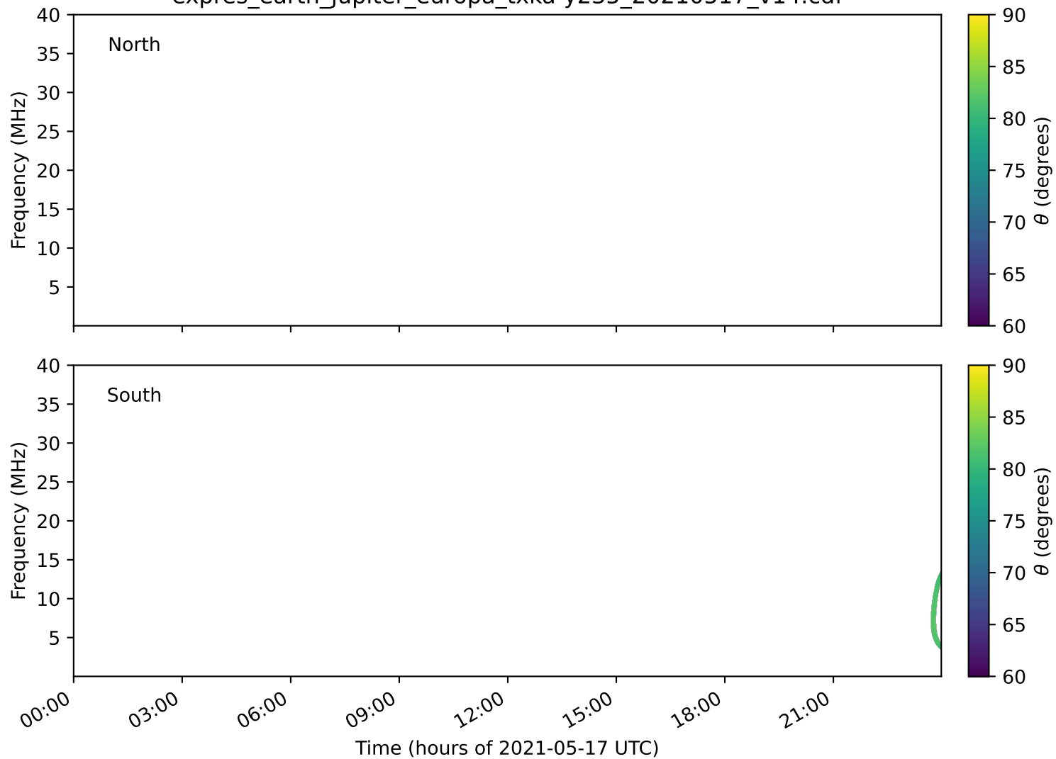
expres_earth_jupiter_europa_txka-y235_20210517_v14.cdf
