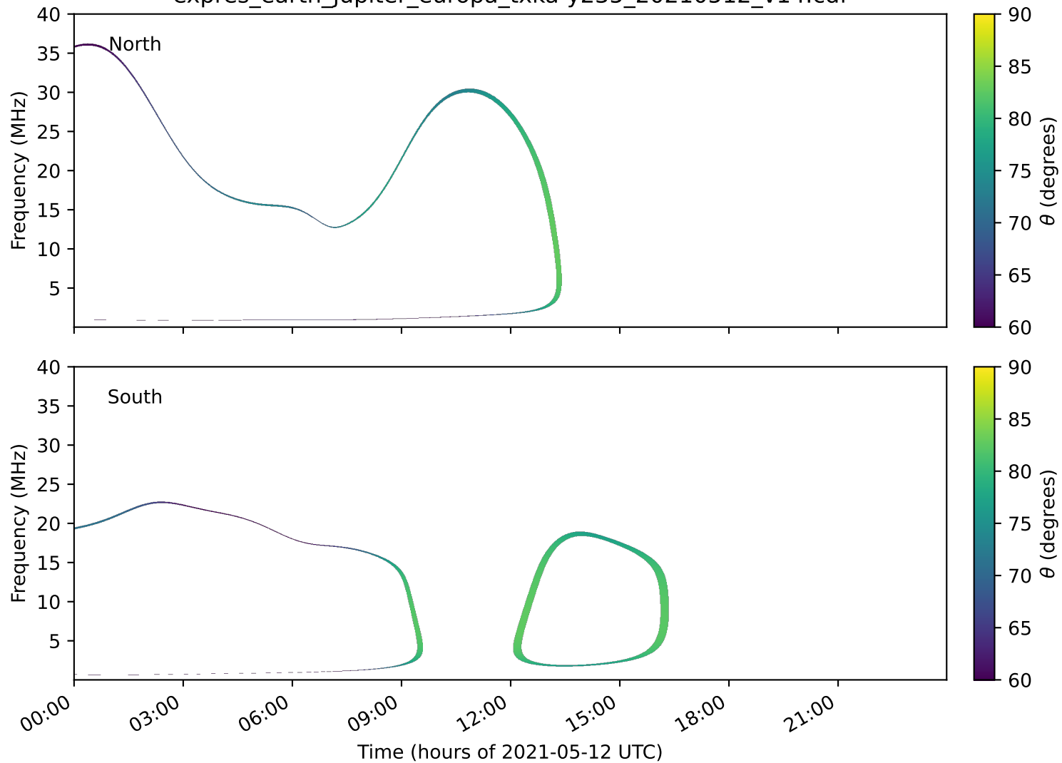
expres_earth_jupiter_europa_txka-y235_20210512_v14.cdf
