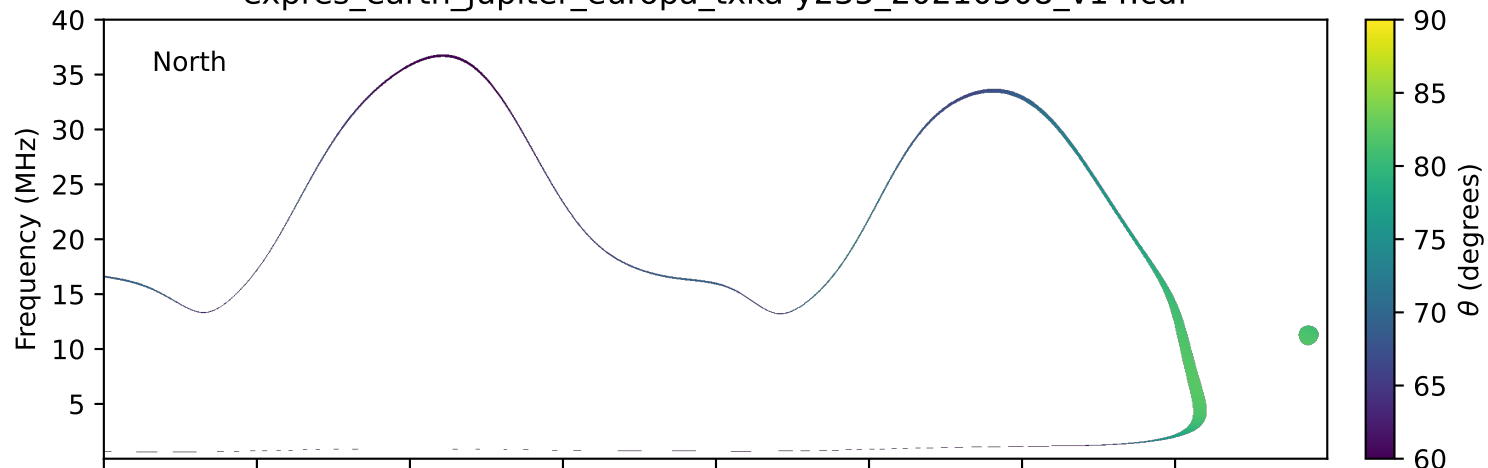
expres_earth_jupiter_europa_txka-y235_20210508_v14.cdf
