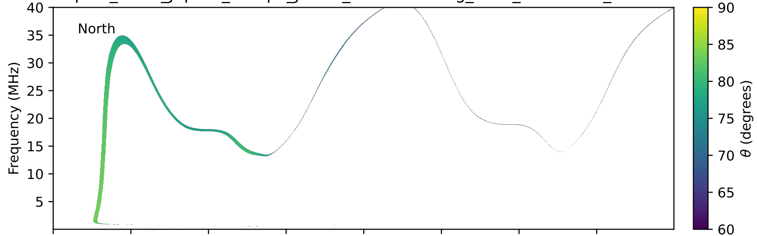
expres_earth_jupiter_europa_jrm33_lossc-wid1deg_3kev_20210511_v11.cdf
