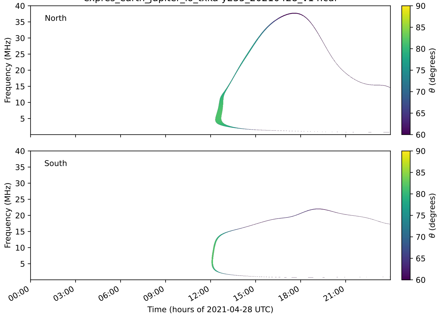
expres_earth_jupiter_io_txka-y235_20210428_v14.cdf
