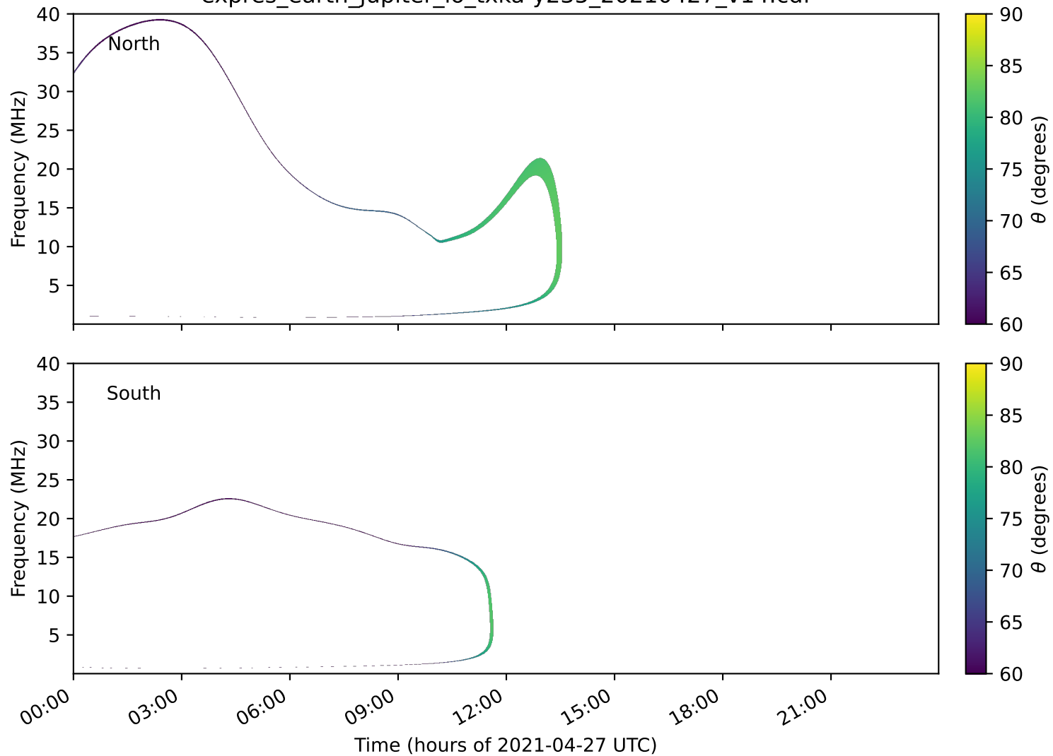
expres_earth_jupiter_io_txka-y235_20210427_v14.cdf
