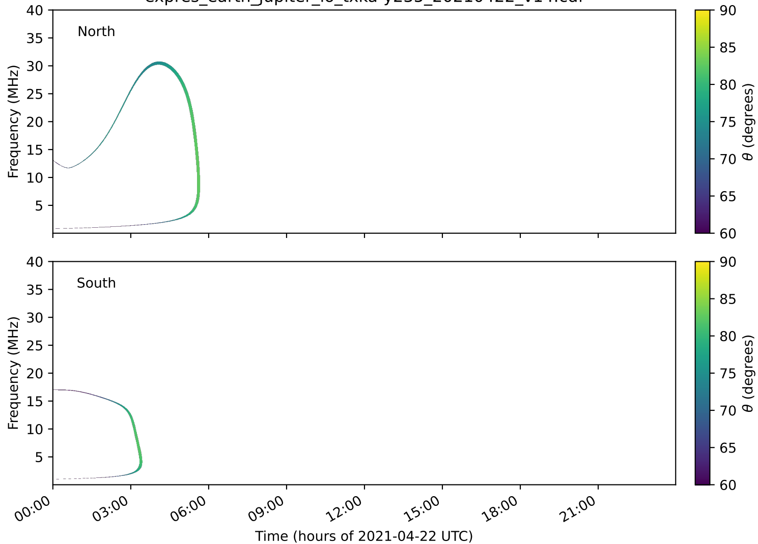
expres_earth_jupiter_io_txka-y235_20210422_v14.cdf
