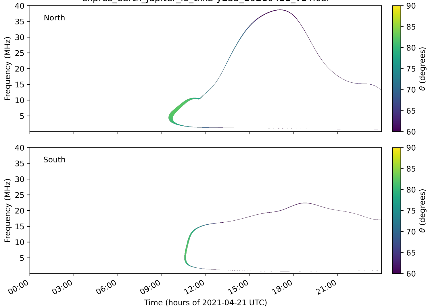
expres_earth_jupiter_io_txka-y235_20210421_v14.cdf
