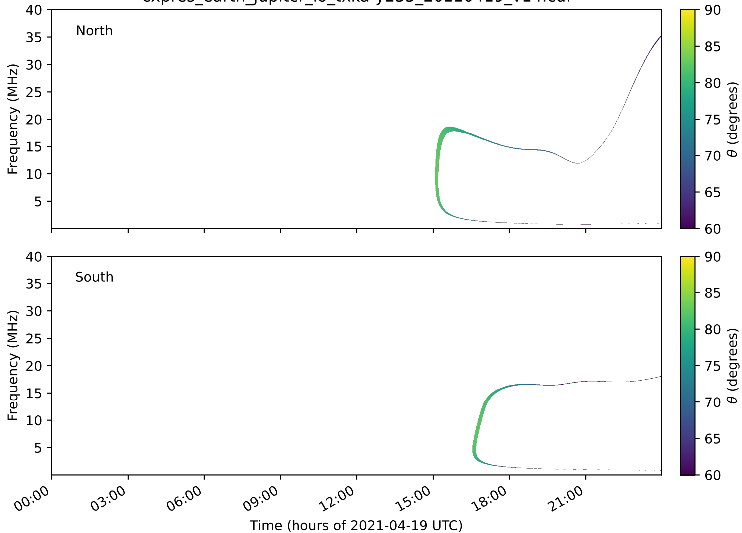
expres_earth_jupiter_io_txka-y235_20210419_v14.cdf
