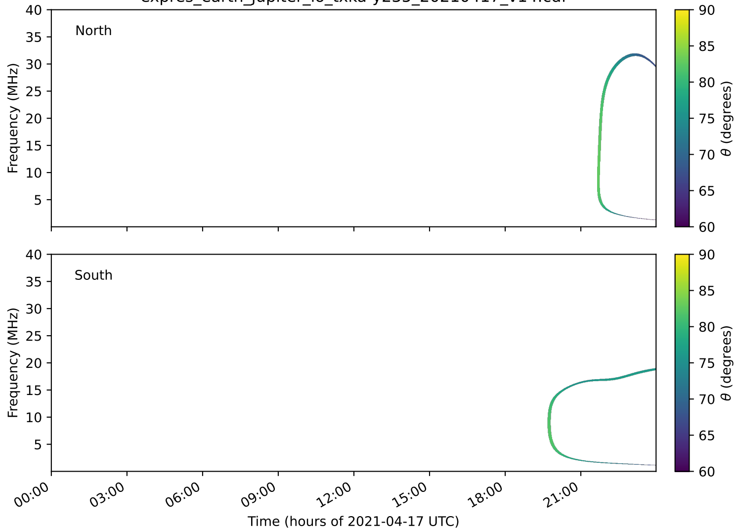
expres_earth_jupiter_io_txka-y235_20210417_v14.cdf
