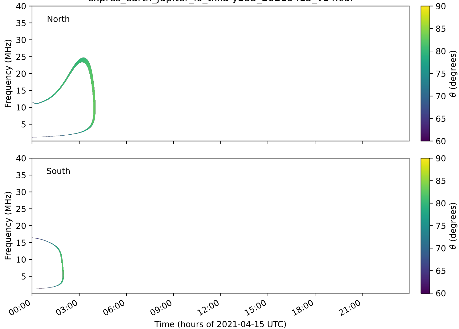
expres_earth_jupiter_io_txka-y235_20210415_v14.cdf
