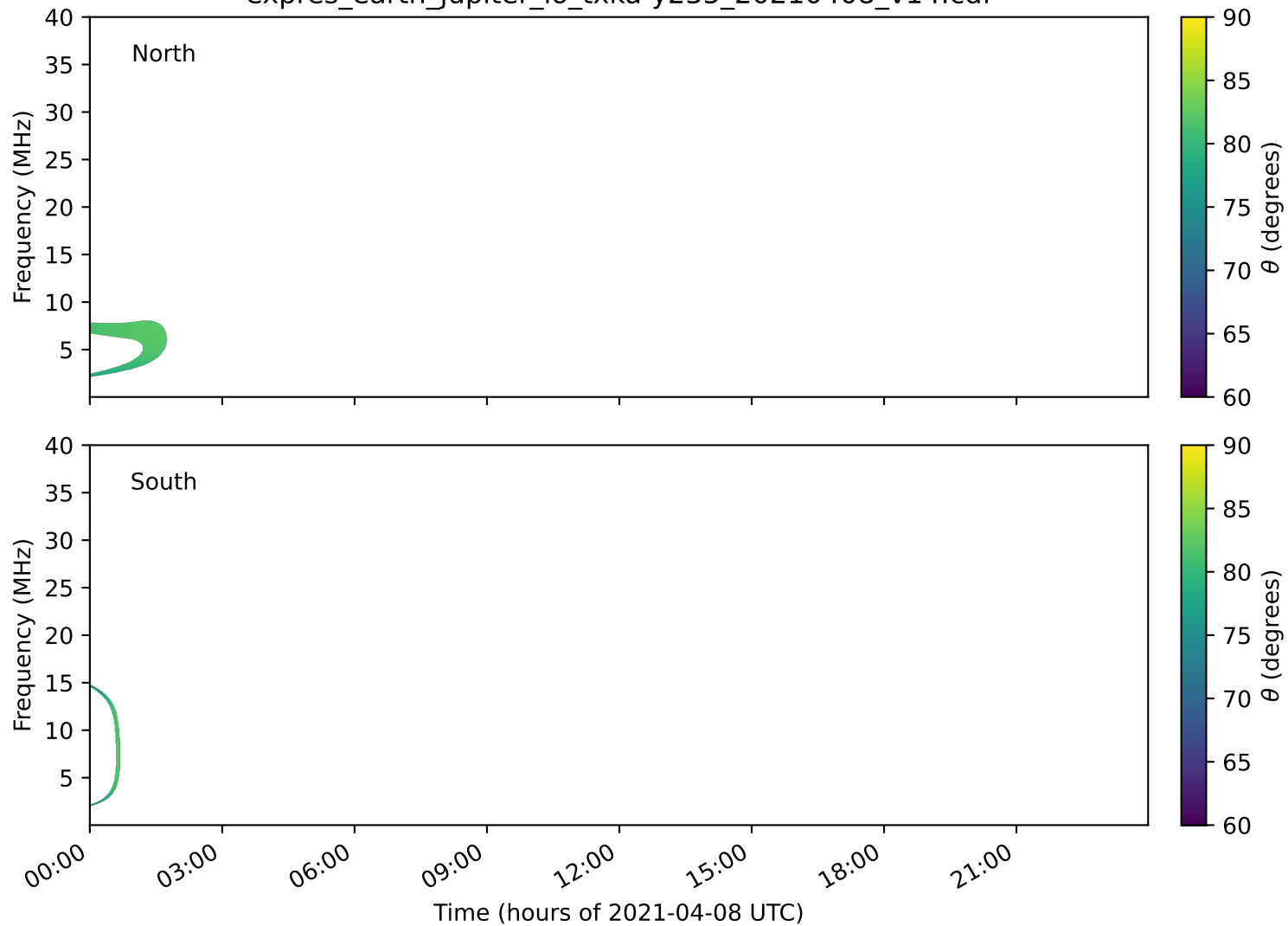
expres_earth_jupiter_io_txka-y235_20210408_v14.cdf
