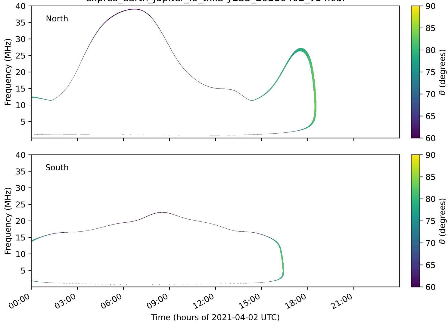
expres_earth_jupiter_io_txka-y235_20210402_v14.cdf
