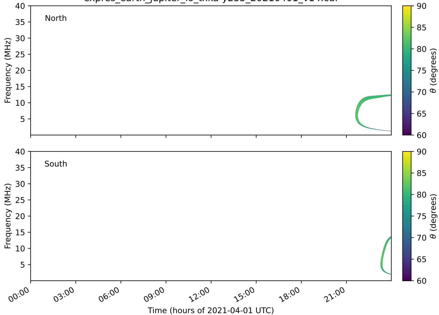
expres_earth_jupiter_io_txka-y235_20210401_v14.cdf
