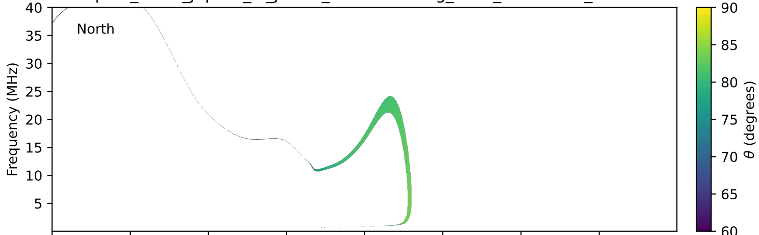
expres_earth_jupiter_io_jrm33_lossc-wid1deg_3kev_20210427_v11.cdf
