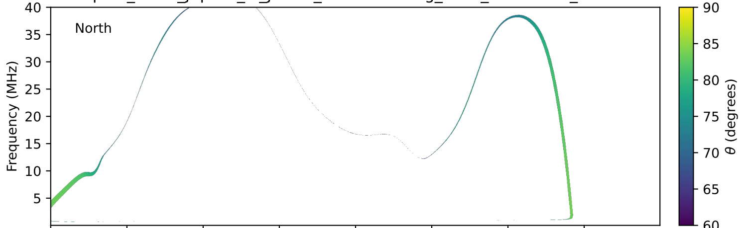
expres_earth_jupiter_io_jrm33_lossc-wid1deg_3kev_20210409_v11.cdf
