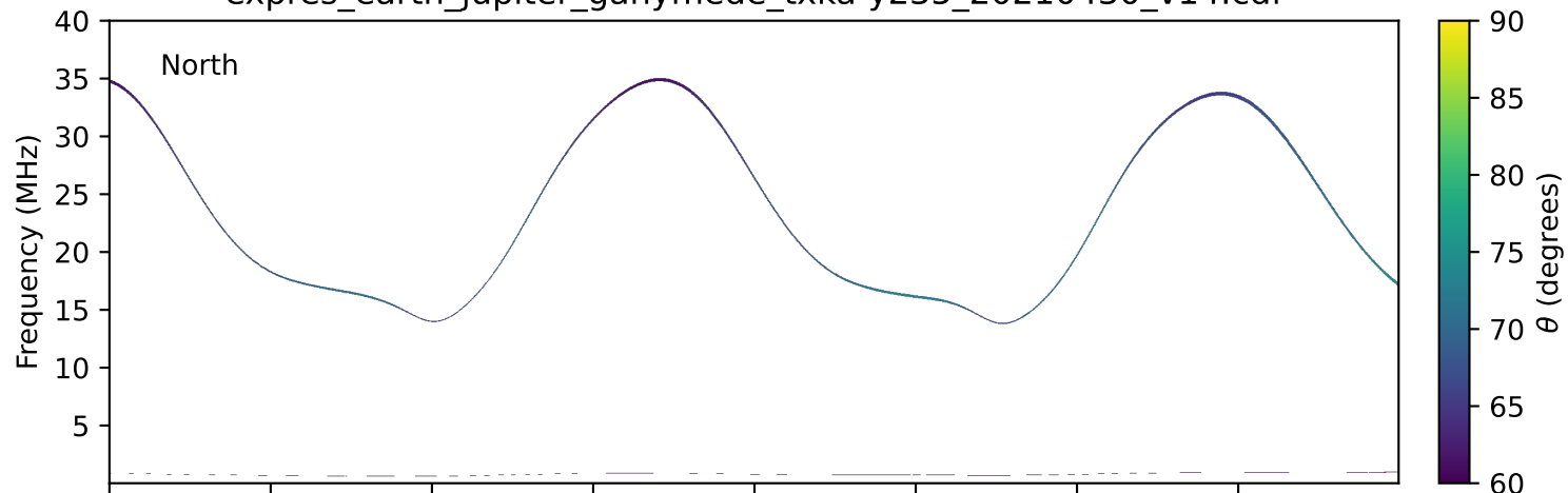
expres_earth_jupiter_ganymede_txka-y235_20210430_v14.cdf
