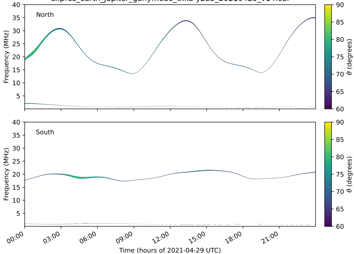
expres_earth_jupiter_ganymede_txka-y235_20210429_v14.cdf
