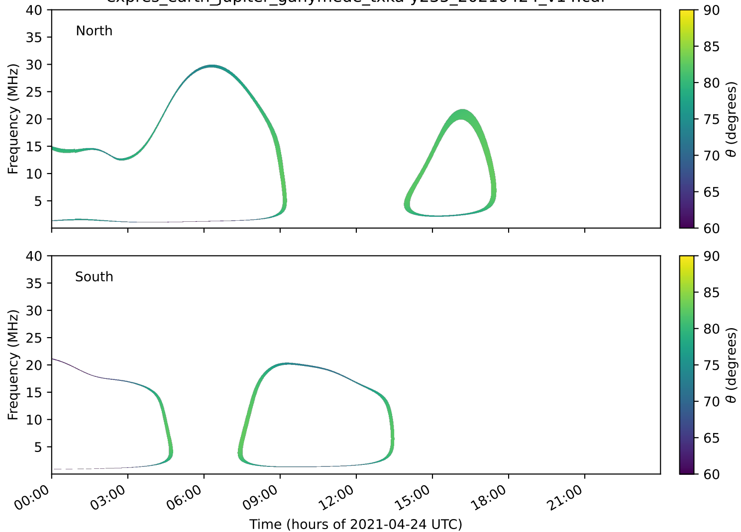
expres_earth_jupiter_ganymede_txka-y235_20210424_v14.cdf
