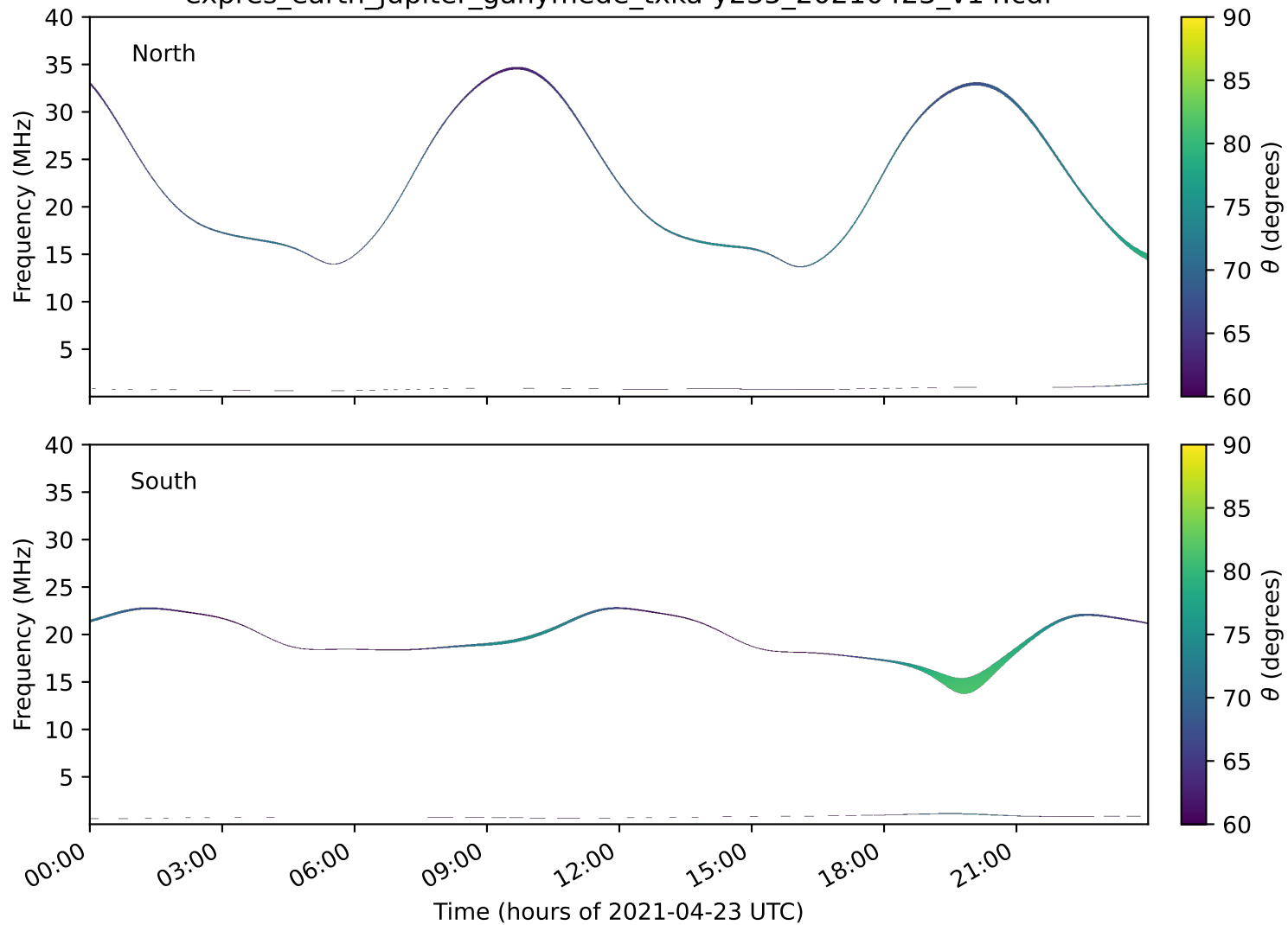
expres_earth_jupiter_ganymede_txka-y235_20210423_v14.cdf
