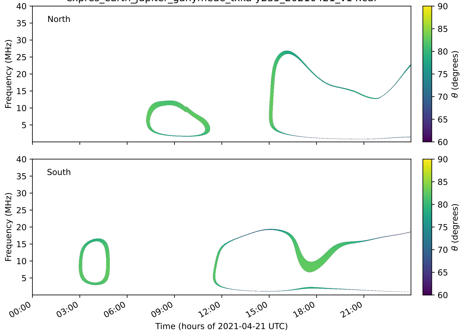
expres_earth_jupiter_ganymede_txka-y235_20210421_v14.cdf
