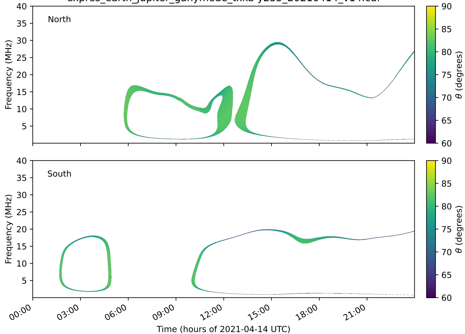
expres_earth_jupiter_ganymede_txka-y235_20210414_v14.cdf
