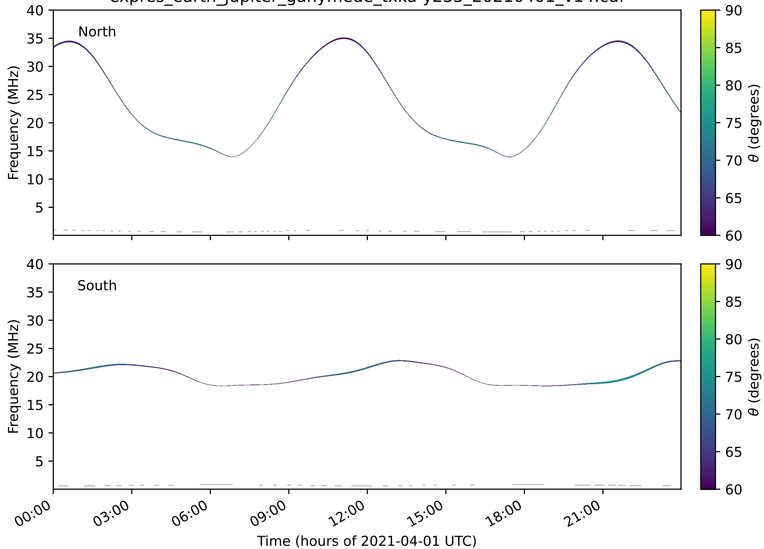
expres_earth_jupiter_ganymede_txka-y235_20210401_v14.cdf
