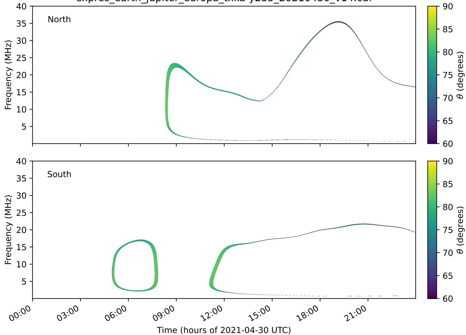
expres_earth_jupiter_europa_txka-y235_20210430_v14.cdf
