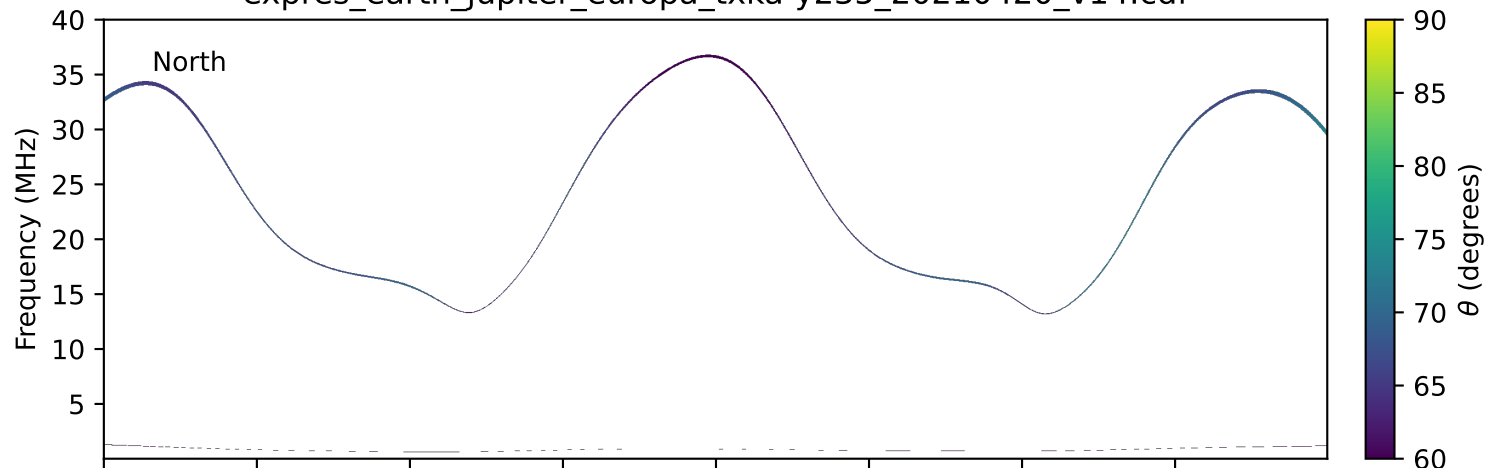
expres_earth_jupiter_europa_txka-y235_20210420_v14.cdf
