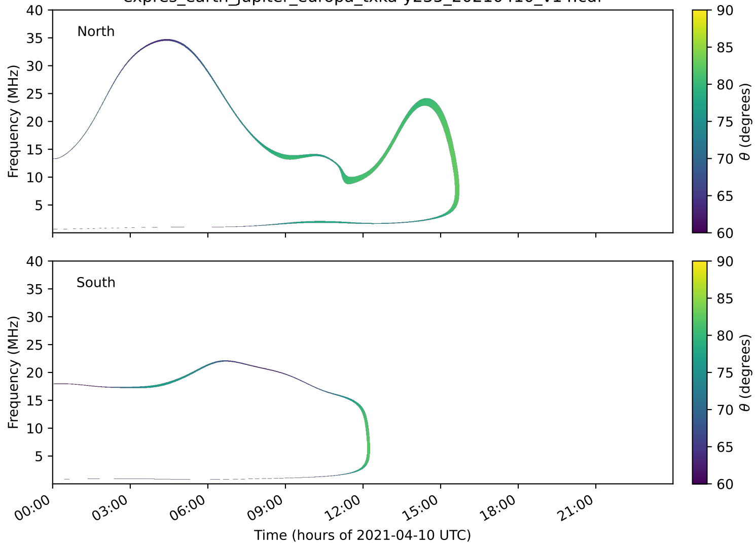
expres_earth_jupiter_europa_txka-y235_20210410_v14.cdf
