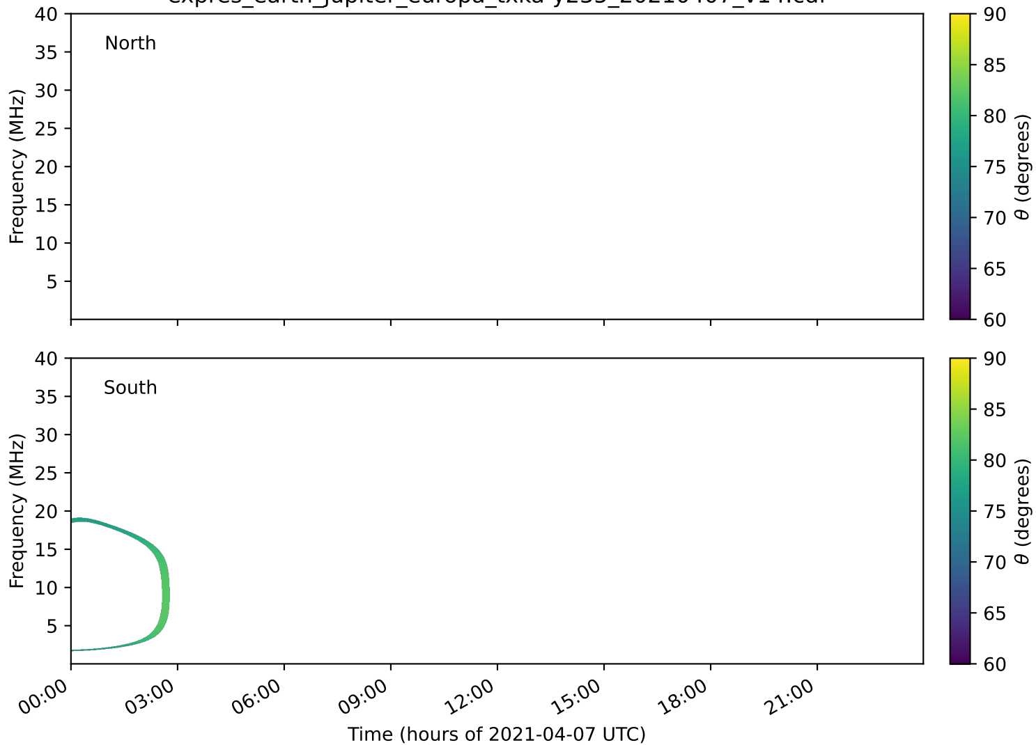
expres_earth_jupiter_europa_txka-y235_20210407_v14.cdf
