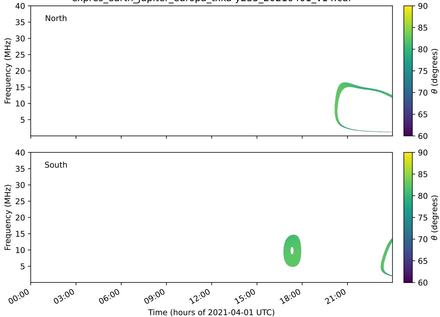
expres_earth_jupiter_europa_txka-y235_20210401_v14.cdf
