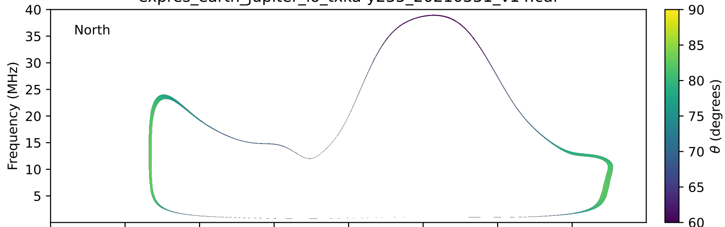
expres_earth_jupiter_io_txka-y235_20210331_v14.cdf
