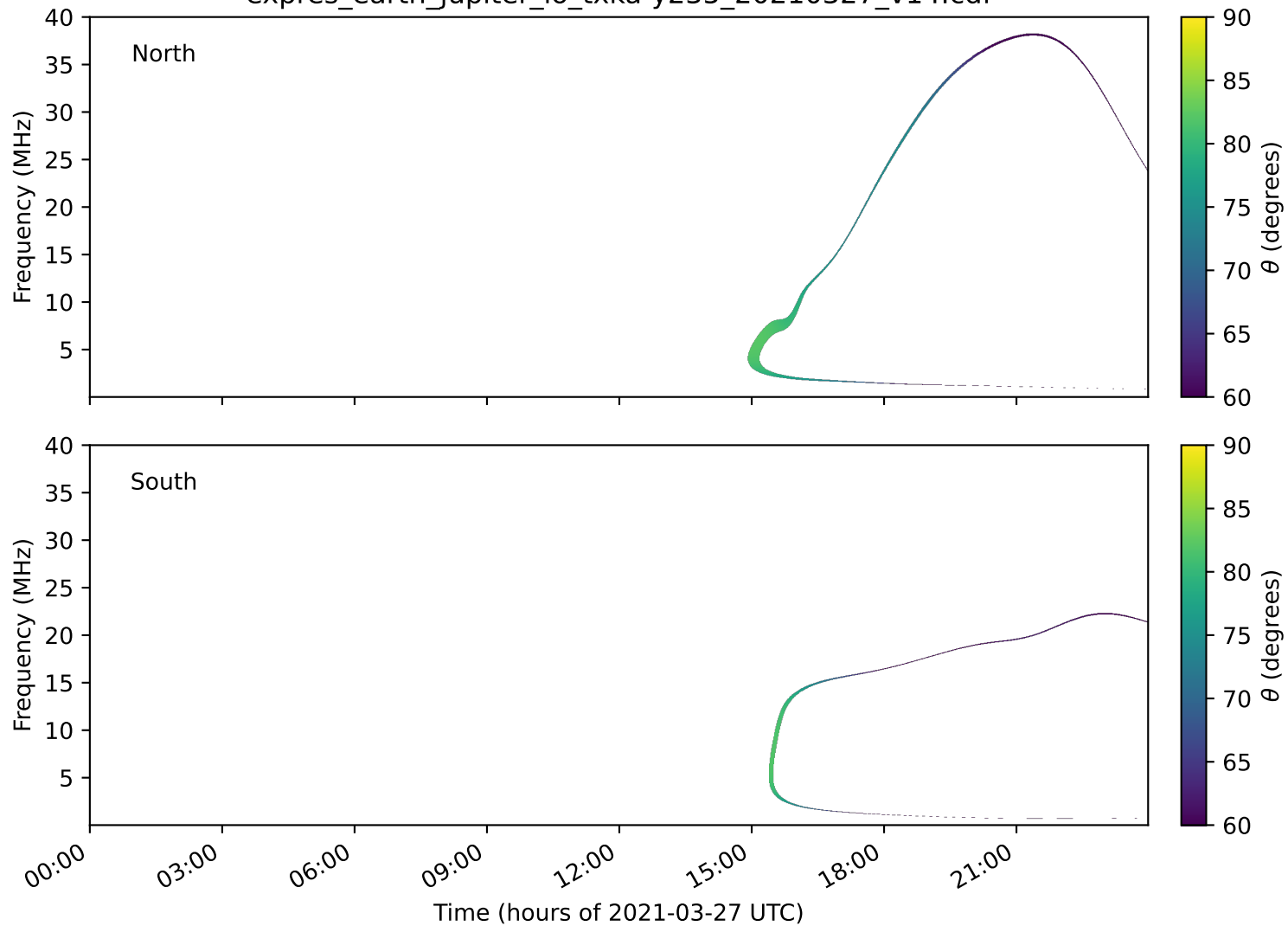
expres_earth_jupiter_io_txka-y235_20210327_v14.cdf
