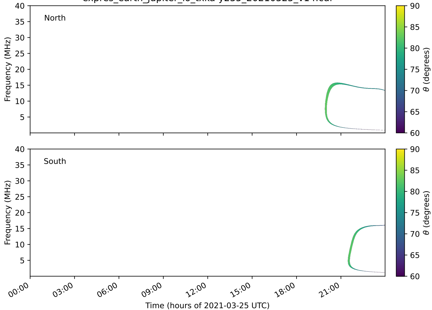
expres_earth_jupiter_io_txka-y235_20210325_v14.cdf
