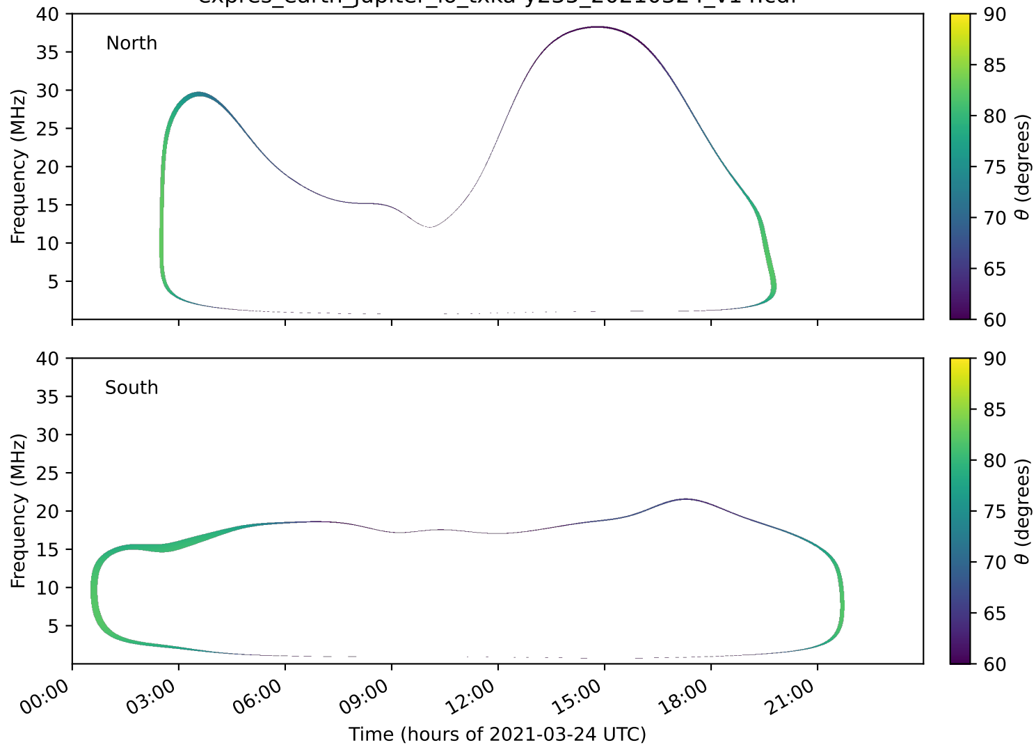
expres_earth_jupiter_io_txka-y235_20210324_v14.cdf
