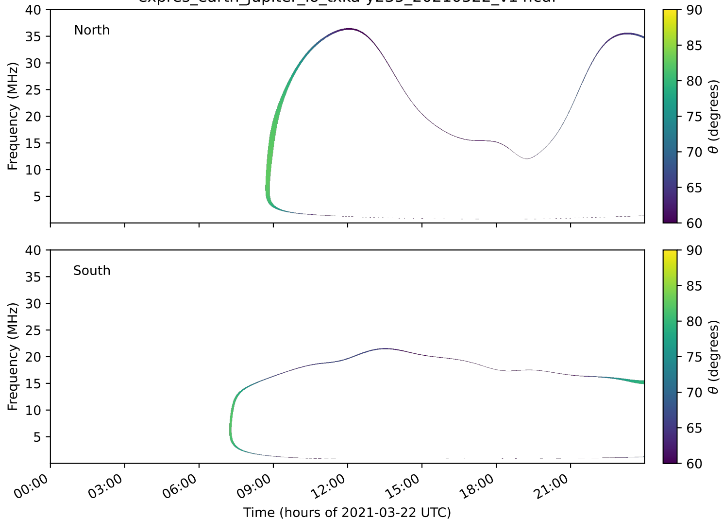
expres_earth_jupiter_io_txka-y235_20210322_v14.cdf
