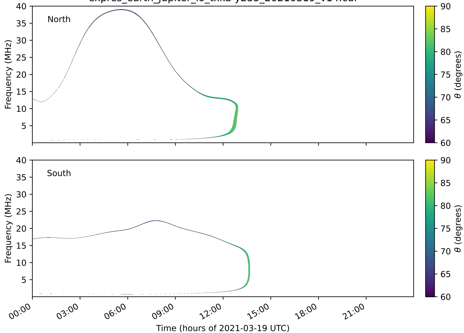
expres_earth_jupiter_io_txka-y235_20210319_v14.cdf
