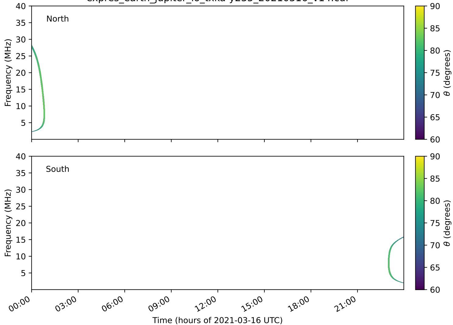
expres_earth_jupiter_io_txka-y235_20210316_v14.cdf
