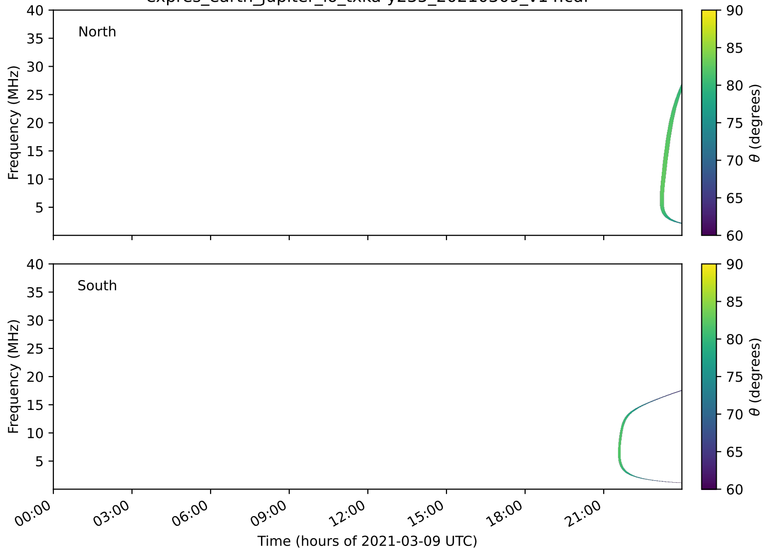
expres_earth_jupiter_io_txka-y235_20210309_v14.cdf
