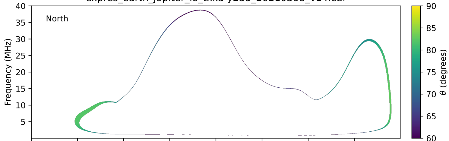
expres_earth_jupiter_io_txka-y235_20210308_v14.cdf
