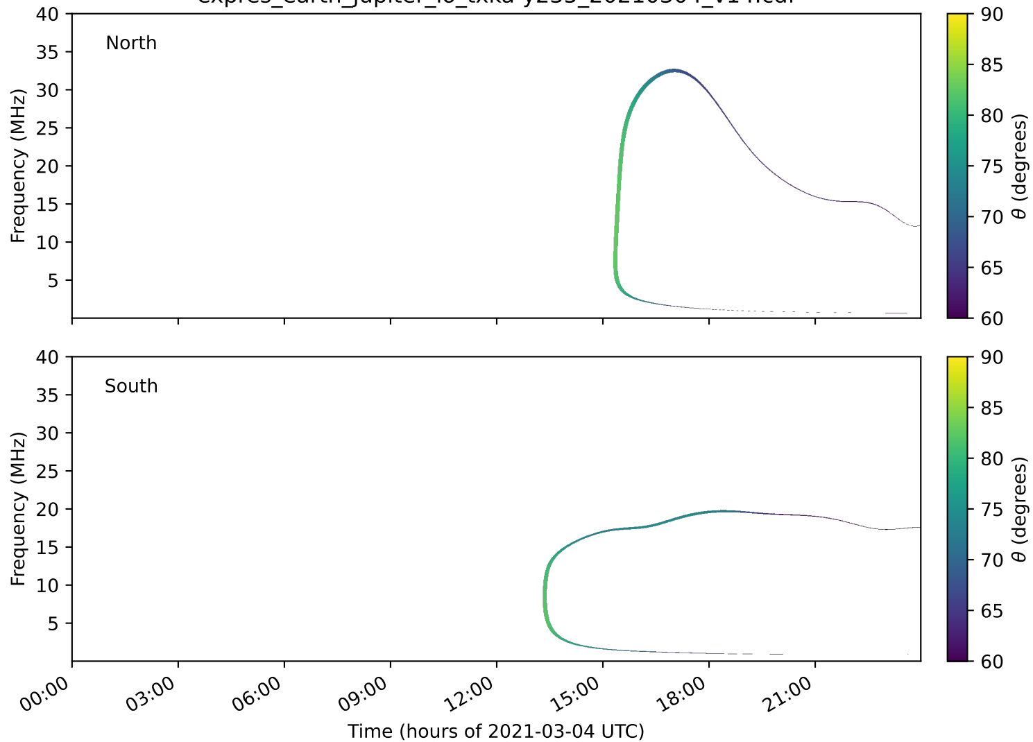
expres_earth_jupiter_io_txka-y235_20210304_v14.cdf
