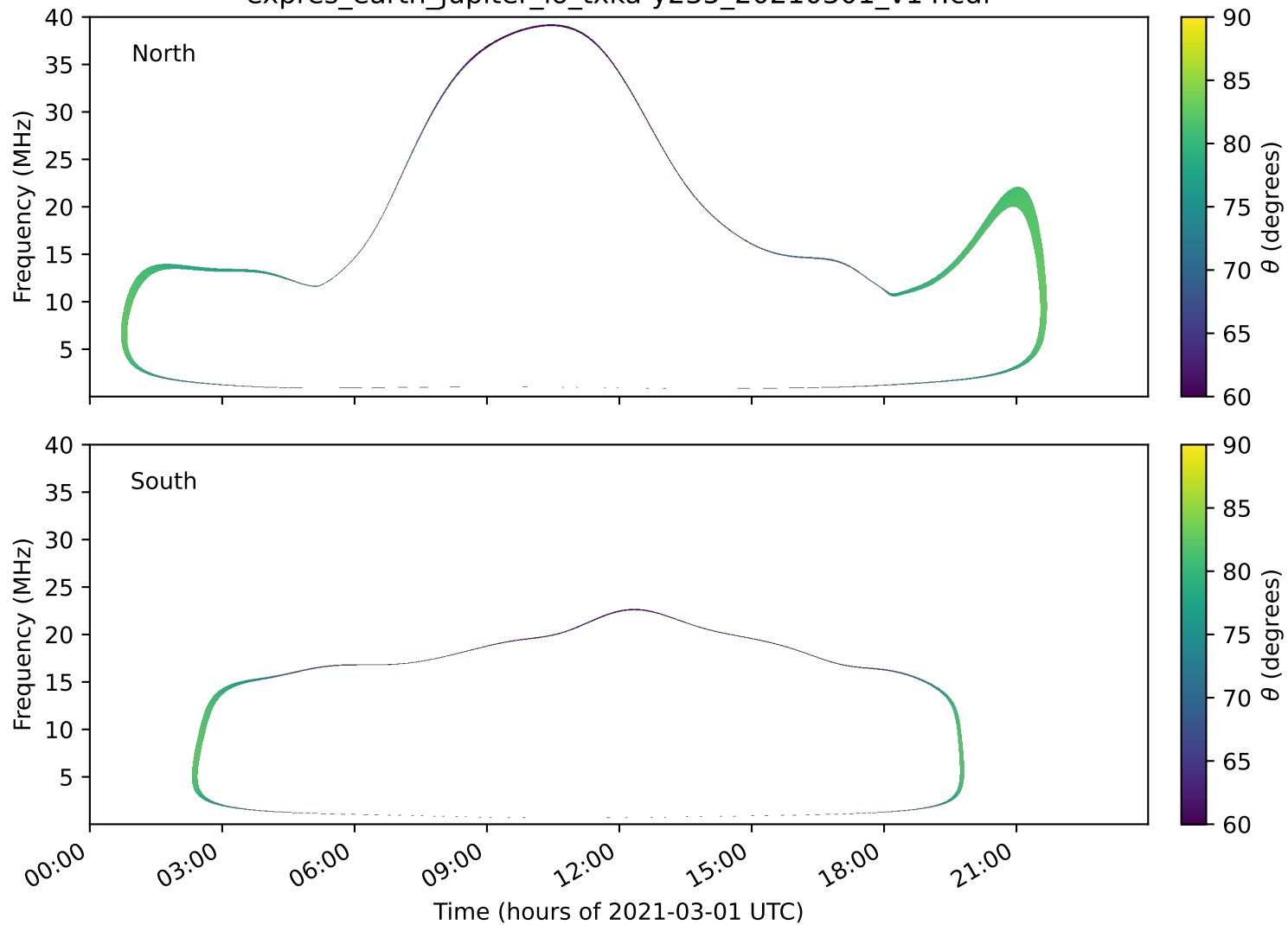
expres_earth_jupiter_io_txka-y235_20210301_v14.cdf
