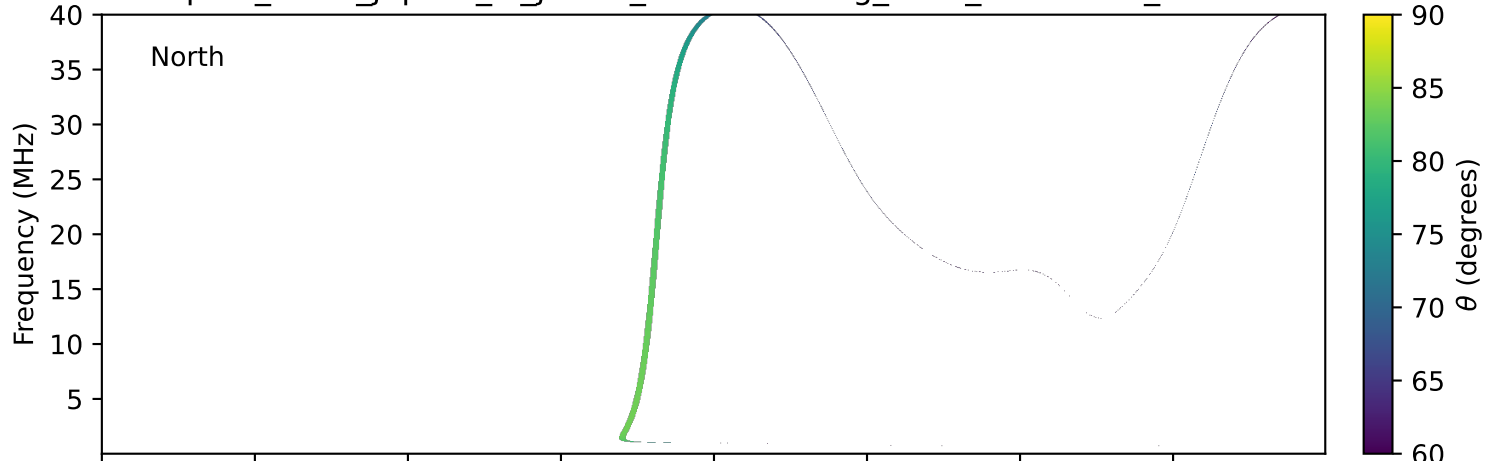
expres_earth_jupiter_io_jrm33_lossc-wid1deg_3kev_20210329_v11.cdf
