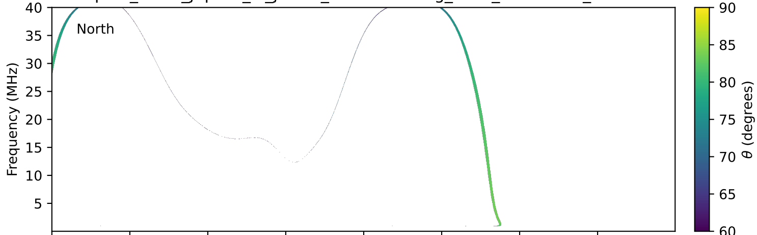
expres_earth_jupiter_io_jrm33_lossc-wid1deg_3kev_20210310_v11.cdf
