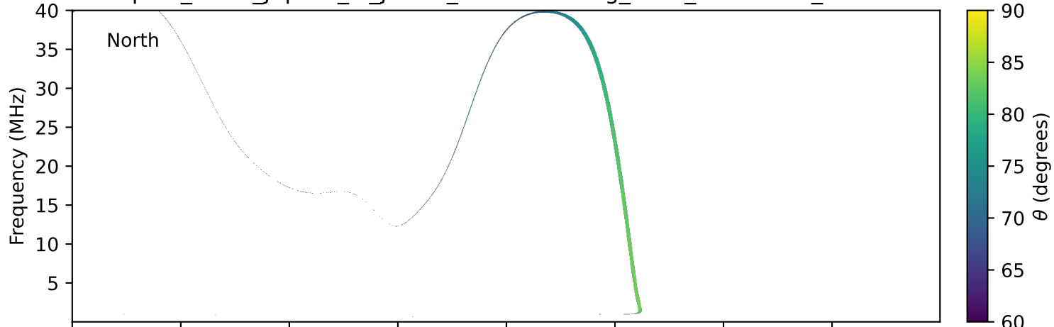
expres_earth_jupiter_io_jrm33_lossc-wid1deg_3kev_20210303_v11.cdf
