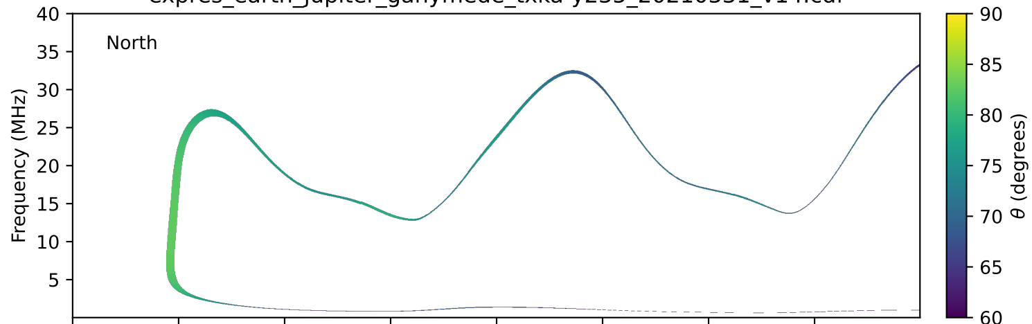
expres_earth_jupiter_ganymede_txka-y235_20210331_v14.cdf
