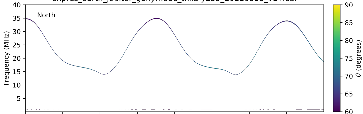
expres_earth_jupiter_ganymede_txka-y235_20210325_v14.cdf
