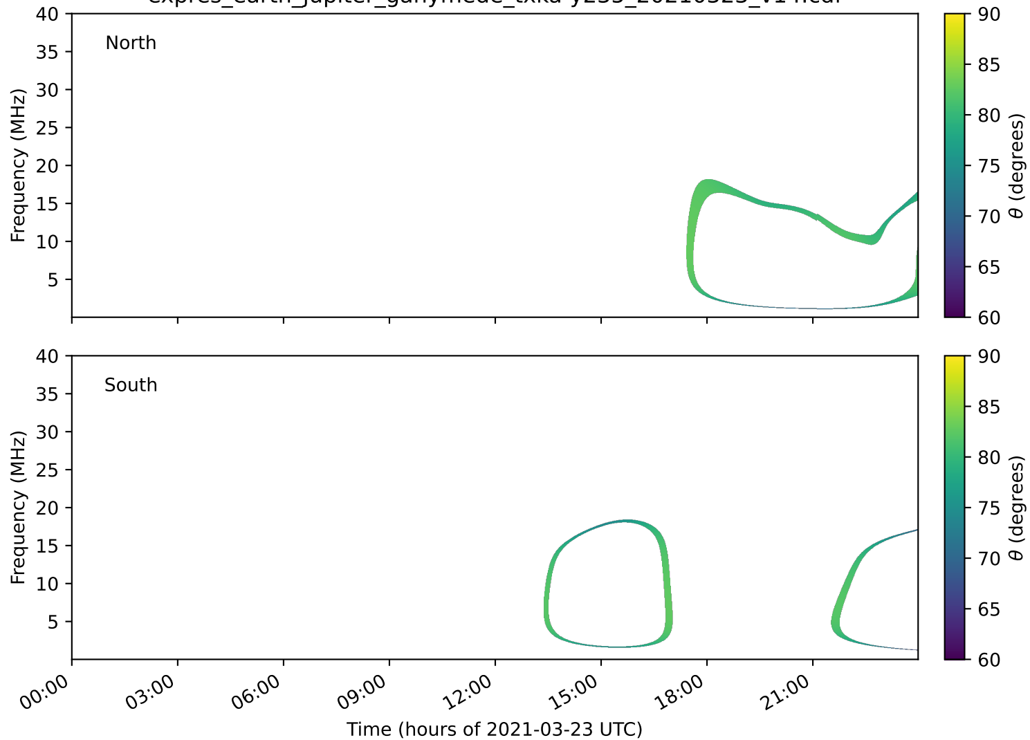
expres_earth_jupiter_ganymede_txka-y235_20210323_v14.cdf
