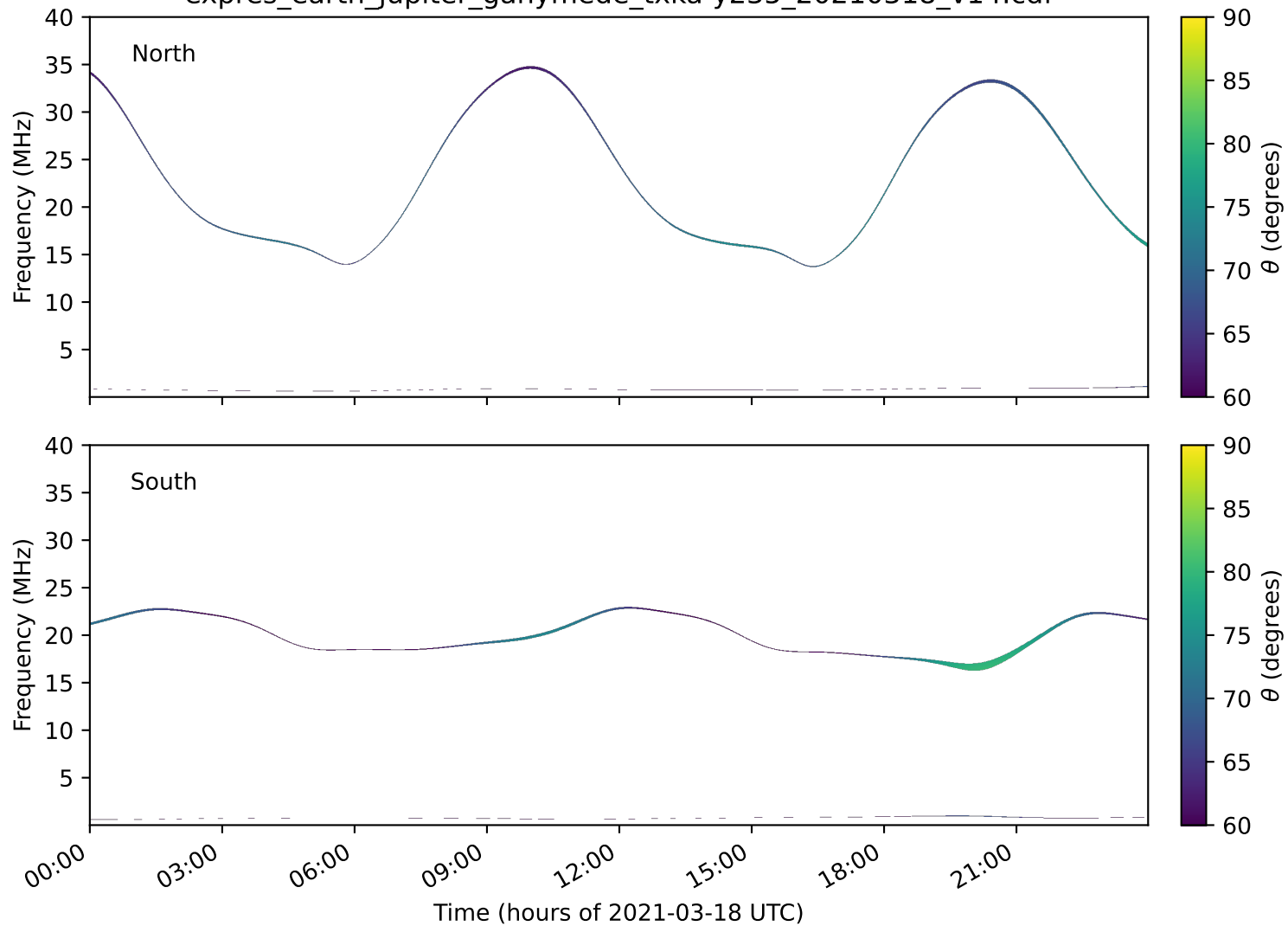
expres_earth_jupiter_ganymede_txka-y235_20210318_v14.cdf
